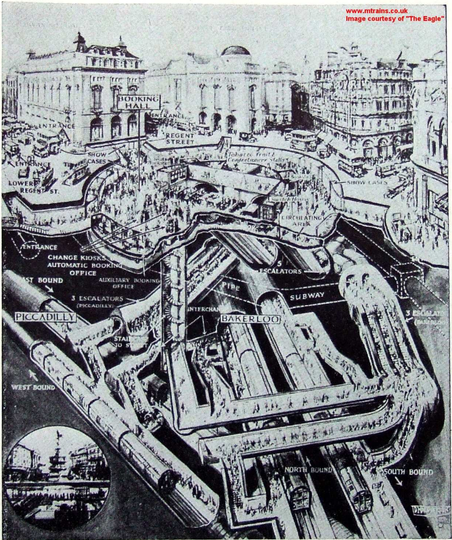
An underground labyrinth. At any tube junction, such as that at Piccadilly Circus, shown in this sectional view, an enormous amount of tunnelling has been necessary, for passages, lifts and escalators, to provide communication between one line and the other, and with the surface.
