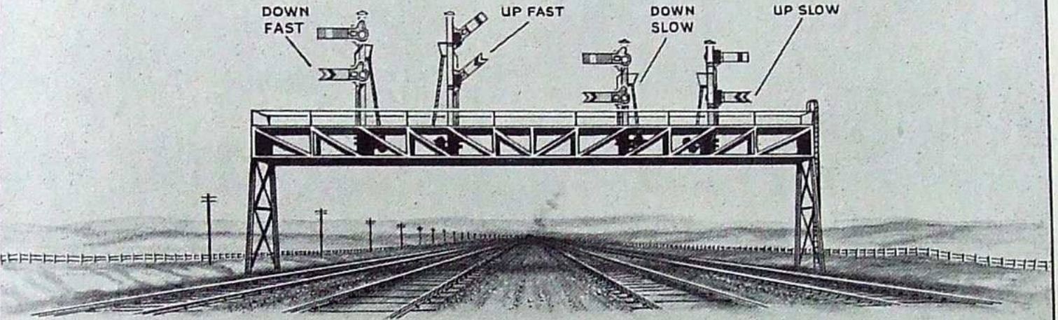
AN 8-ARM UPPER QUADRANT GANTRY. THE SEMAPHORES ALWAYS POINT TO THE LEFT OF THE TRACK THEY CONTROL
