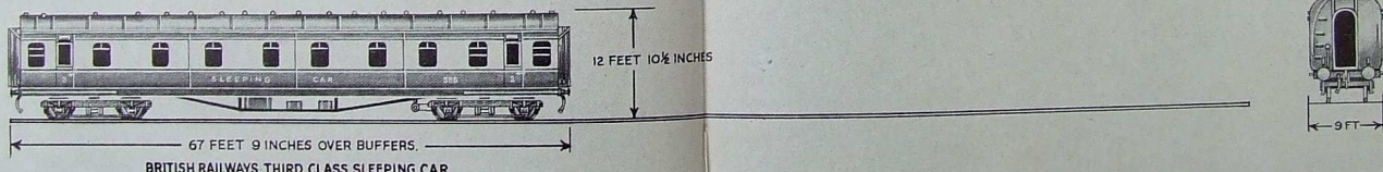
BRITISH RAILWAYS THIRD CLASS SLEEPING CAR
